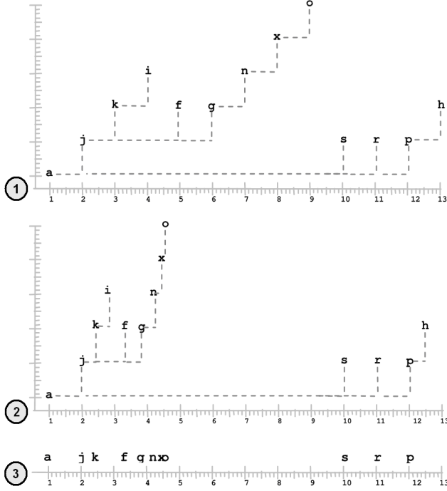
Figure 4. An example of applying continuity scheme
